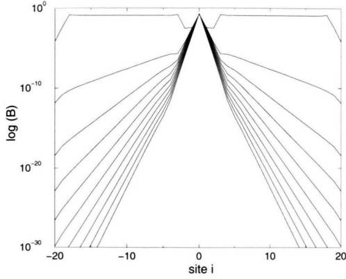
Fig. 1. Spatial decay profile for different couplings c in the lattice described by (1). The parameters are d = 0.05 , h = 0.3 , \omega_0 = 2.25 . From bottom to top, the couplings are c = 0.016 , c = 0.018 , c = 0.020 , c = 0.022 , c = 0.025 , c = 0.028 , c = 0.032 , c = 0.035 , c = 0.040 , c = 0.046 . For couplings above c_{cr} \approx 0.04 the localization property gets lost.
